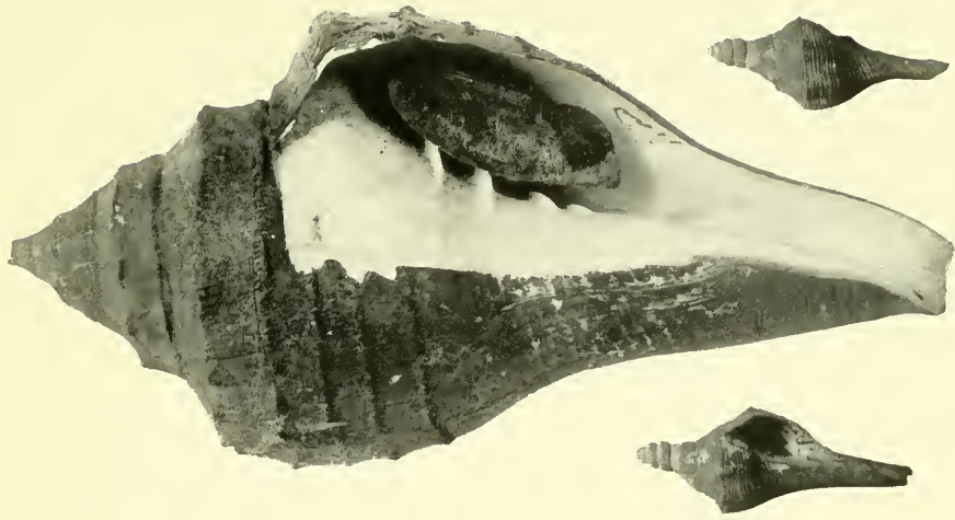
FIG. 2.—ELONGATED VARIETY FROM THE ANDAMAN ISLANDS, ADULT AND 2 VERY YOUNG SPECIMENS. THE LATTER SHOW THE PROTO- CONCH PERSISTING.
